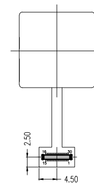
BOTTOM VIEW
